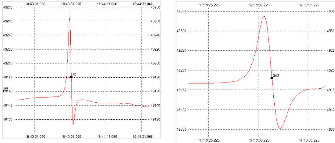
Figure 23: Magnetic anomalies of 151 nT (MT_53)
